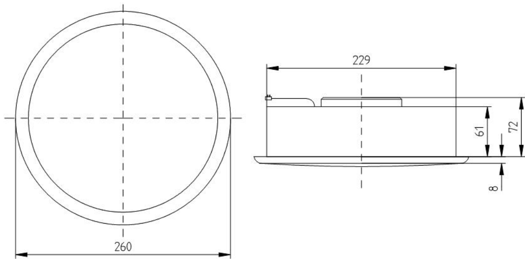
Figure 1: Dimensional drawing LD 6 UE / 229
